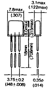
UM-1 Resistance Weld
